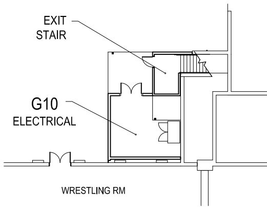
GROUND LEVEL FLOOR PLAN
