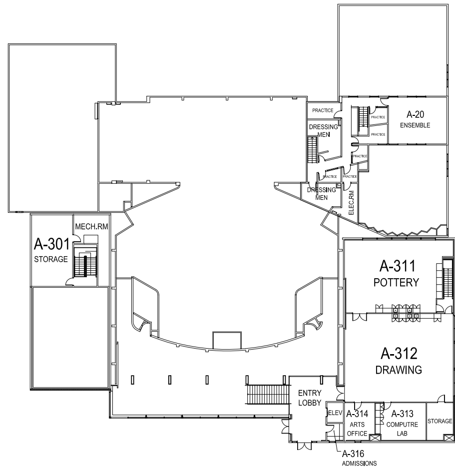
UPER LEVEL FLOOR PLAN
