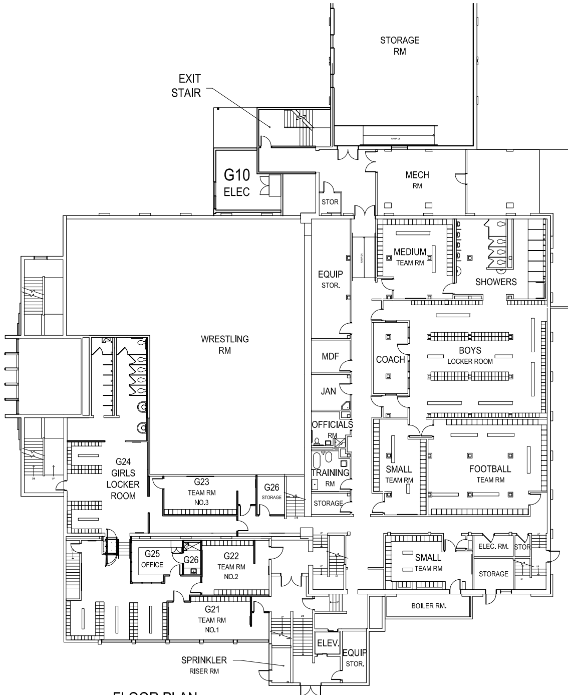
FLOOR PLAN
