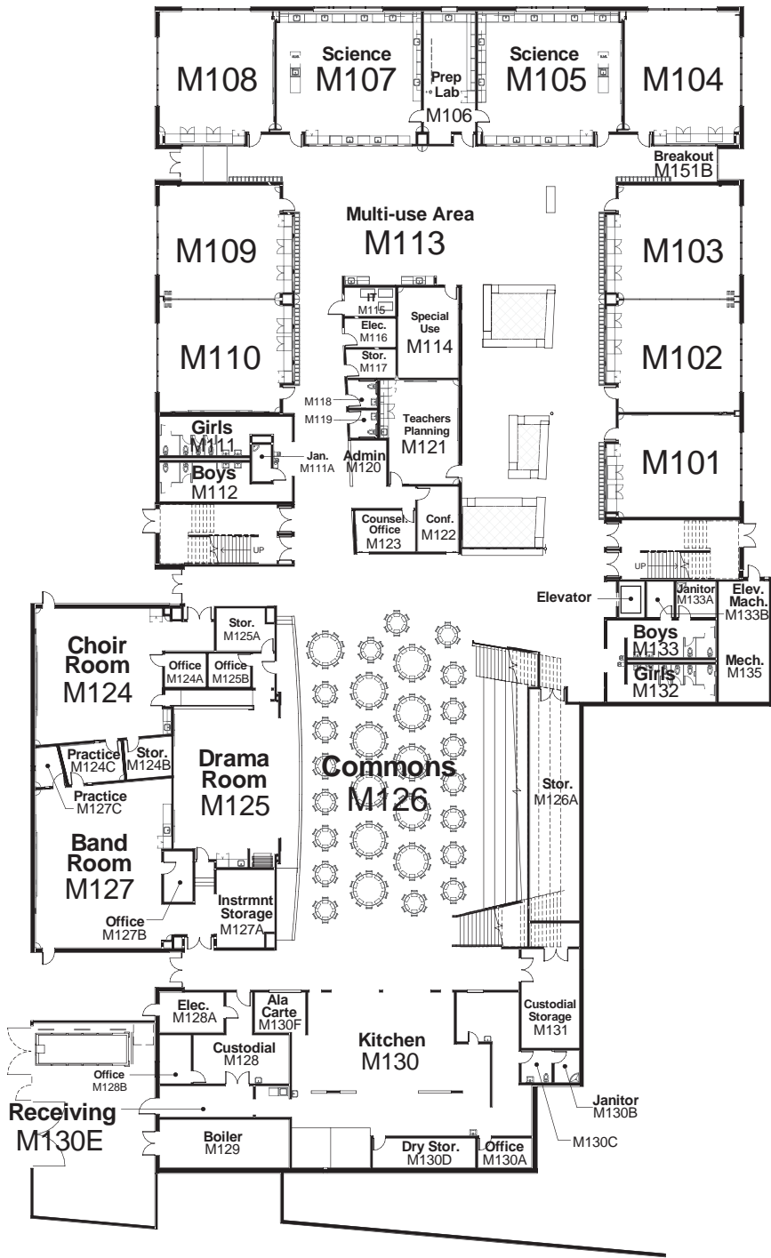
North arrow pointing up. First Level Plan
