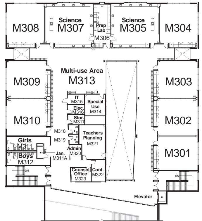
North arrow pointing up. Third Level Plan
